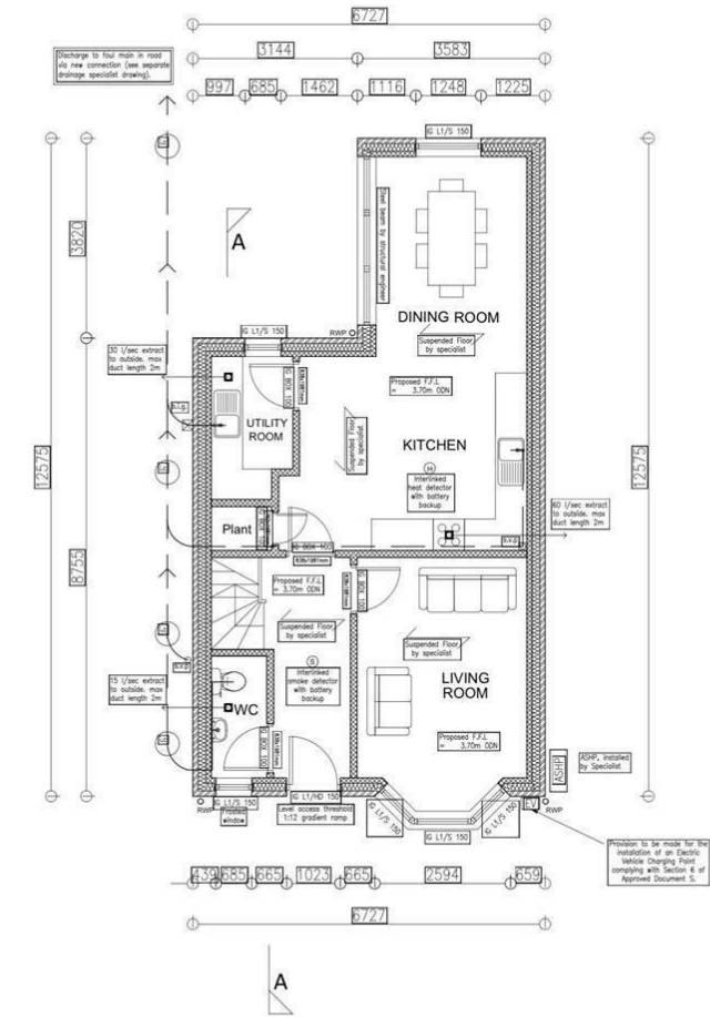
Proposed Ground Floor Plan Scale 1:50
